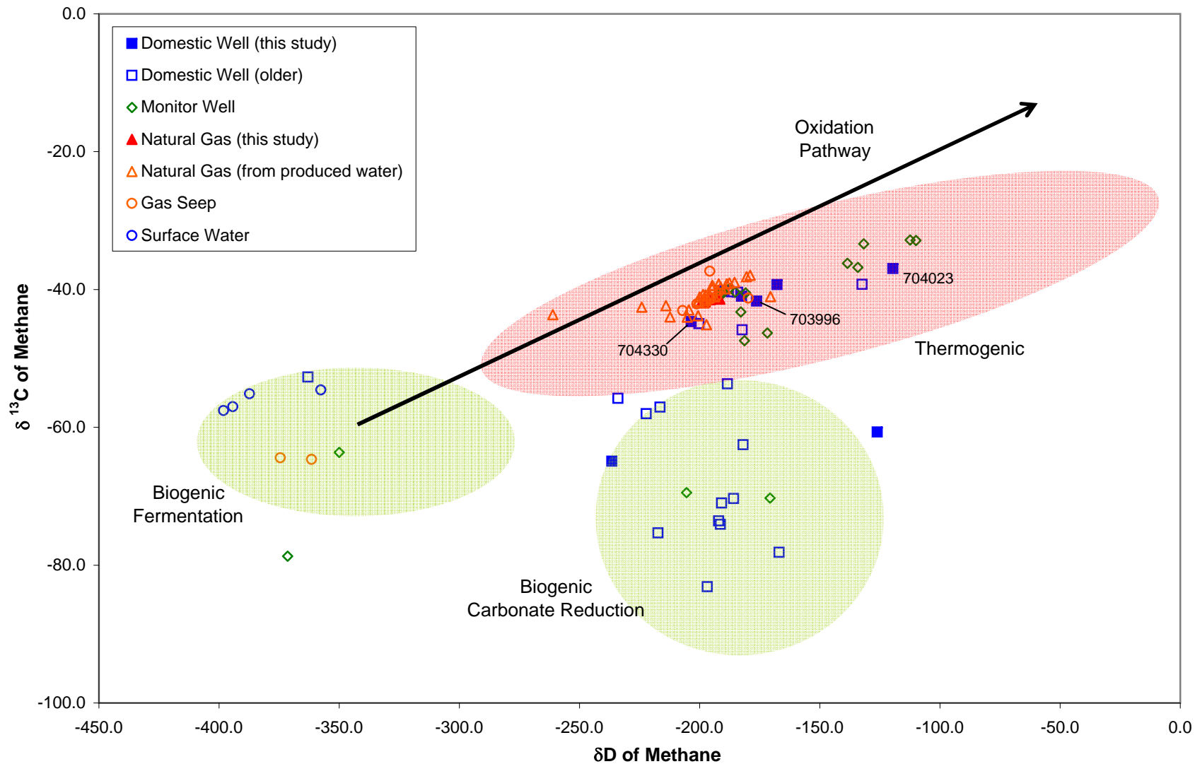
Figure 4.19 Carbon and Hydrogen Isotopes of Methane for Mamm Creek Study Area with Regions of Biogenic and Thermogenic Natural Gases (adapted from Whiticar, 1990).
